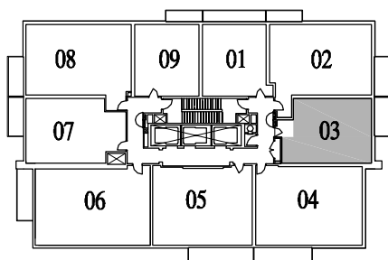
5th-32nd FLOOR PLAN
