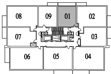
4th-32nd FLOOR PLAN
