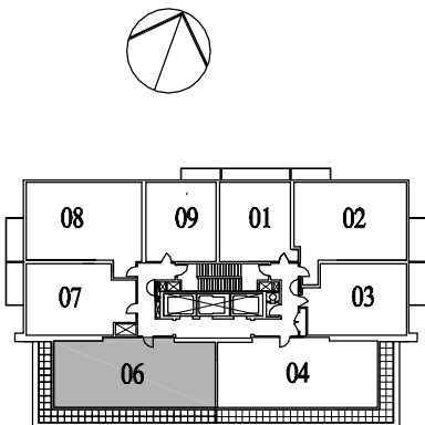
29th FLOOR PLAN
