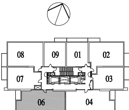
30th FLOOR PLAN
