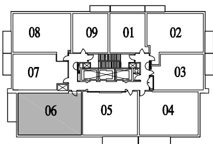
6th-27th FLOOR PLAN
